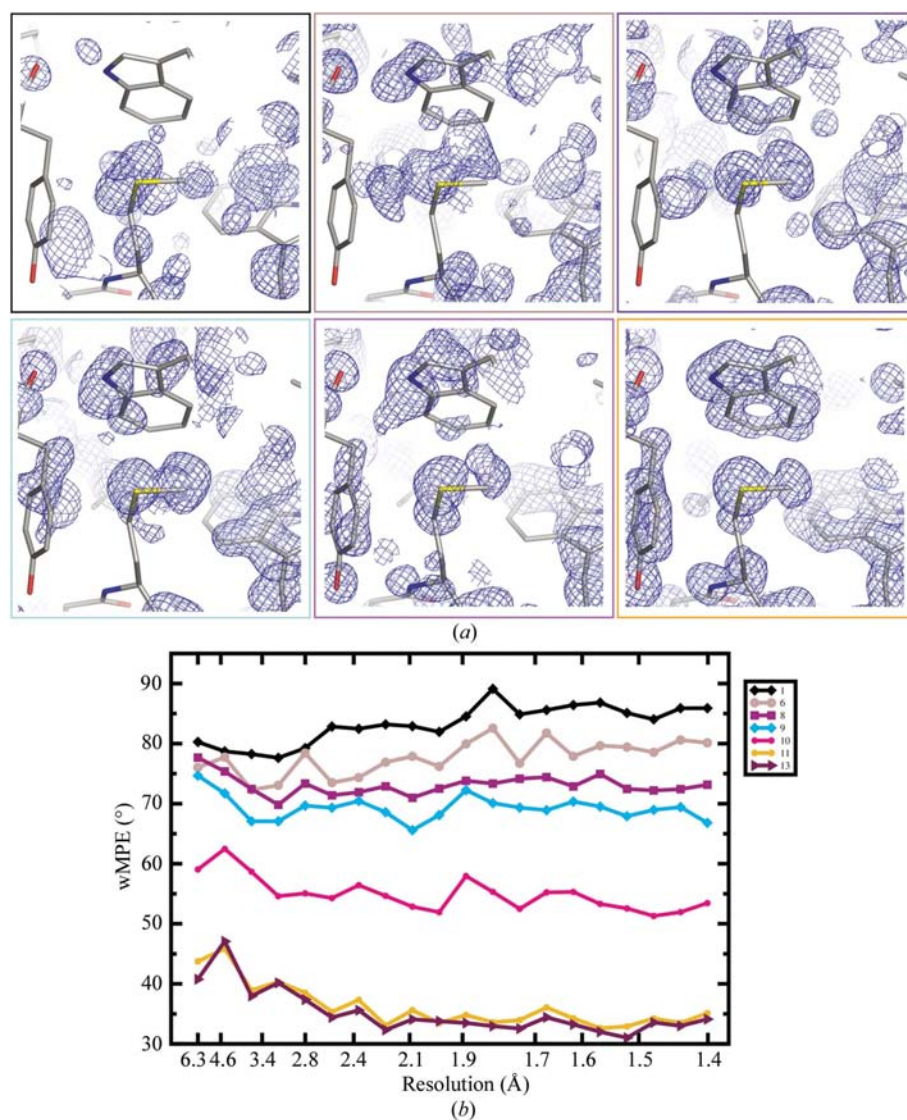
Figure 6 Experimental electron-density maps ( a ) and weighted mean phase errors ( b ) for lysozyme for different subsequent iterations in SHELXE . A total of 13 substructure iterations were made; maps were drawn after iteration Nos. 1, 6, 8, 9, 10 and 11.
